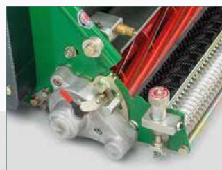
Simple to operate groomer drive engagement
