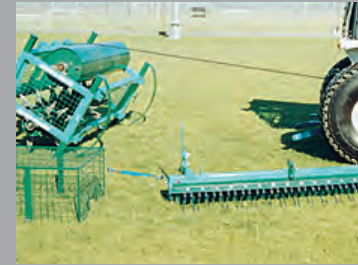
3 Drive tractor forward to roll Double-Quick over.
