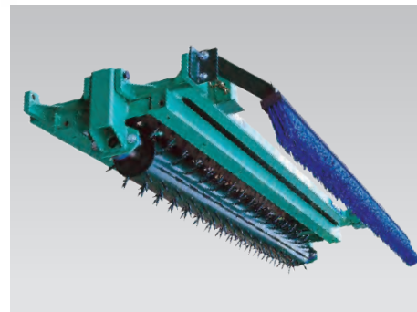
Sarel-Roller Cassette with Rear Dew Brush fits into an existing Maxi-Brush frame.
