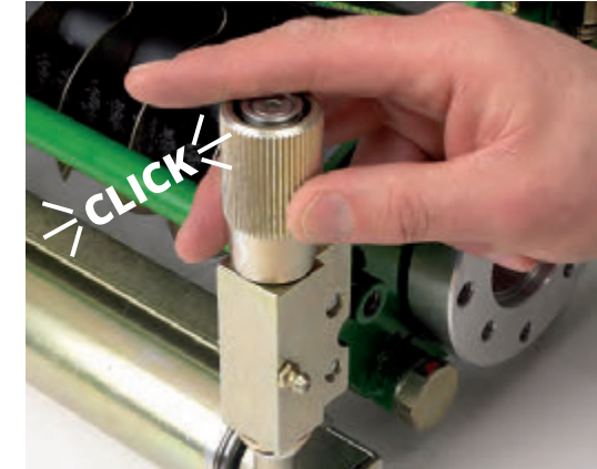
Unique Set By Feel™ height adjustment.
